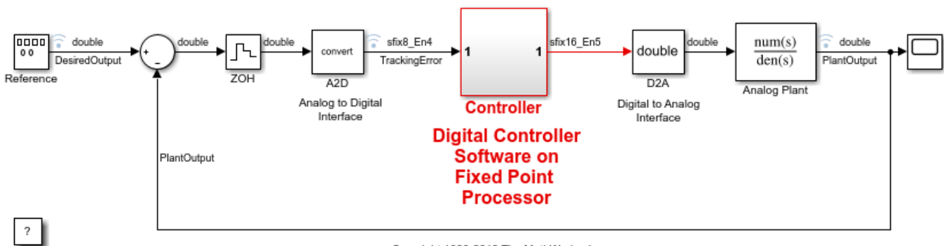
Scaling a Fixed-Point Control Design
